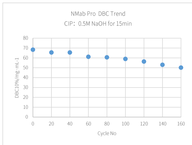
Figure 5. DBC of HCCF that employ harsh CIP treatment (0.5M NaOH exposure for 15min) after each cycle.
