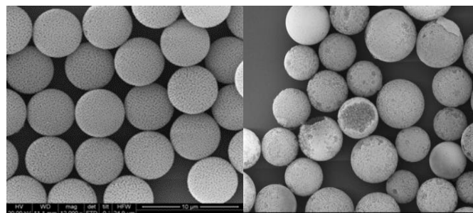
Figure 3. UniHybrid 8-120 C8 (left) and a competitor 8-120 C8 (right) repeatedly loaded column pressure changes and resin breakage by SEM
