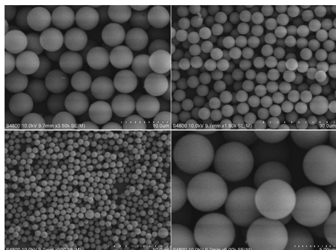
Figure 2. SEM pictures of UniHybrid 8-120 C8 particles
